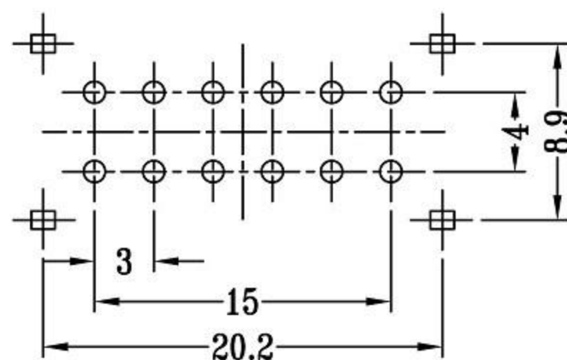
P.C.B LAYOUT BOTTOM VIEW
